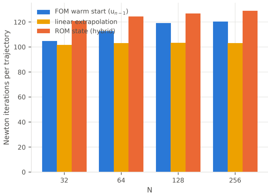
Total Newton iterations (50 steps)
