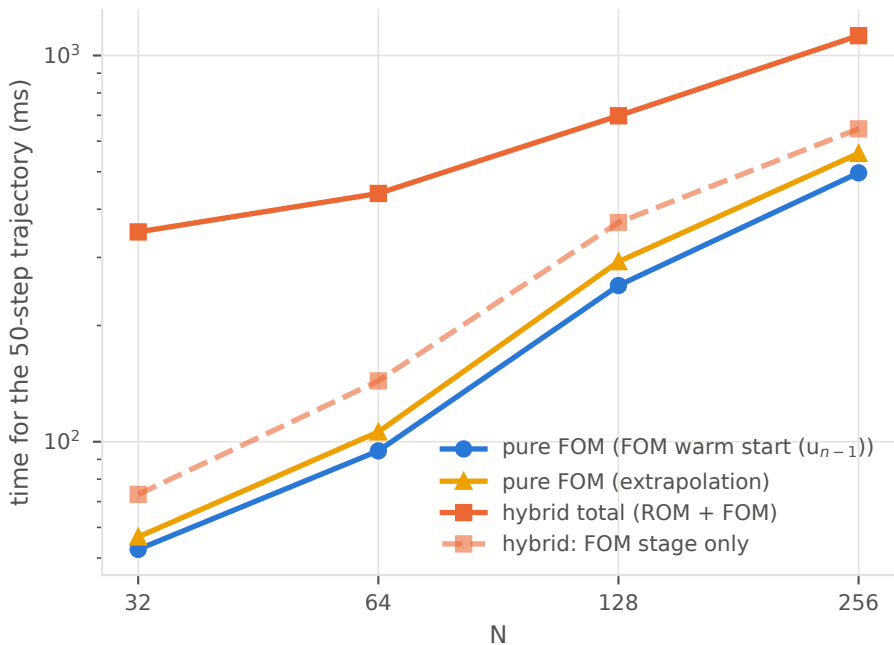
Burgers-2D cost vs mesh ( \tau_{FOM}=1e-10 )
