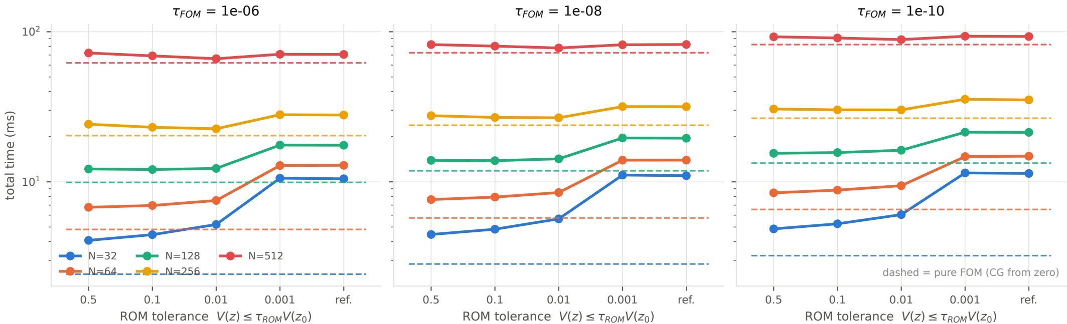
Poisson-2D: hybrid total cost vs the ROM's own stopping tolerance
