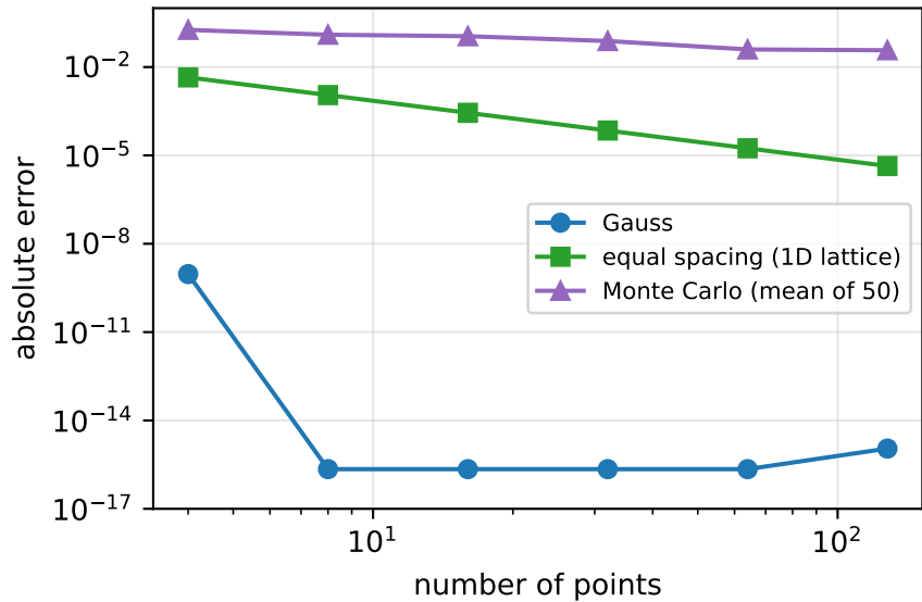
f(x) = e^x (does not vanish at the ends)
