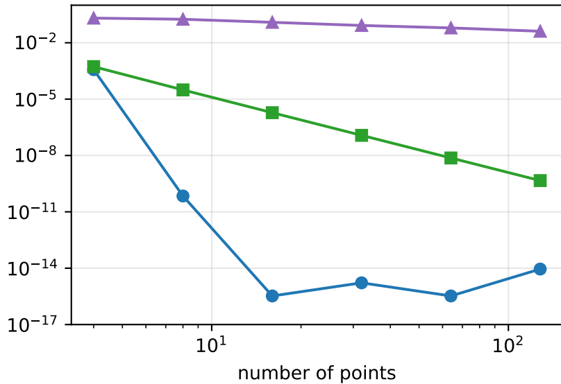
f(x) = \sin^2(\pi x) e^x (vanishes at the ends)
