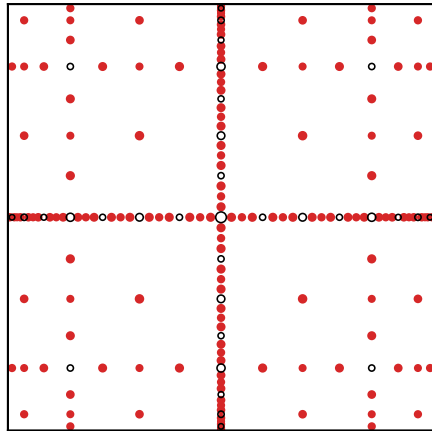
Smolyak level 6 m = 193
