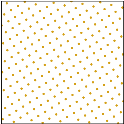
Fibonacci lattice m = 233
