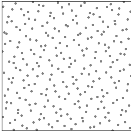
Sobol (scrambled) m = 256
