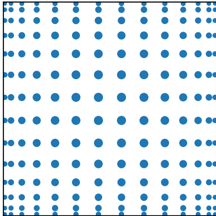
Gauss 14 \times 14 m = 196
