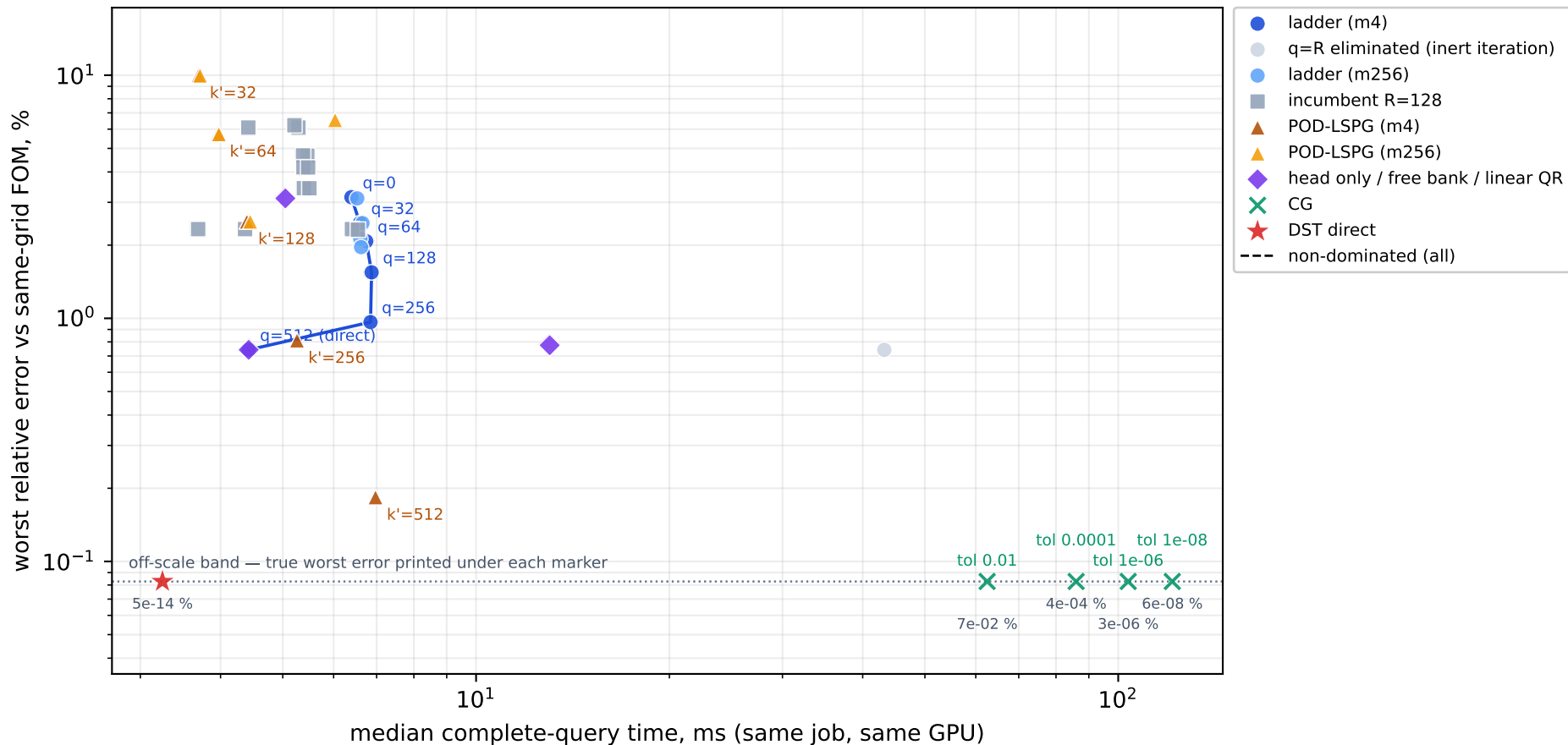
Poisson 2D, 1024 2 intervals: correction ladder against every comparator (one job, one GPU, 12 development sources, 3 timed repetitions)
