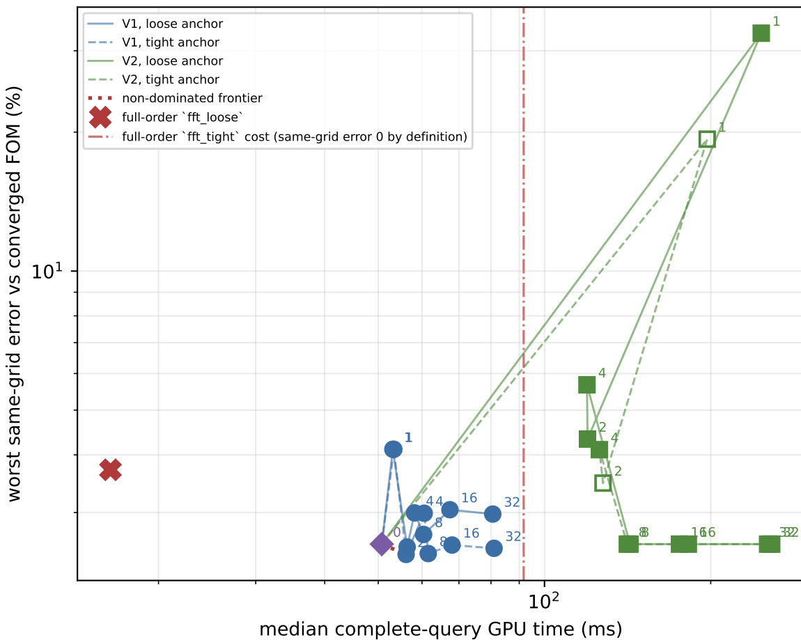
Burgers 2D, 256 intervals (marker: D n=0, o V1, s V2; open = early-stopped)
