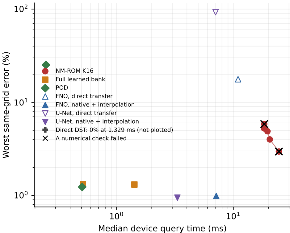
Heat 3D — 64 intervals per axis — development
