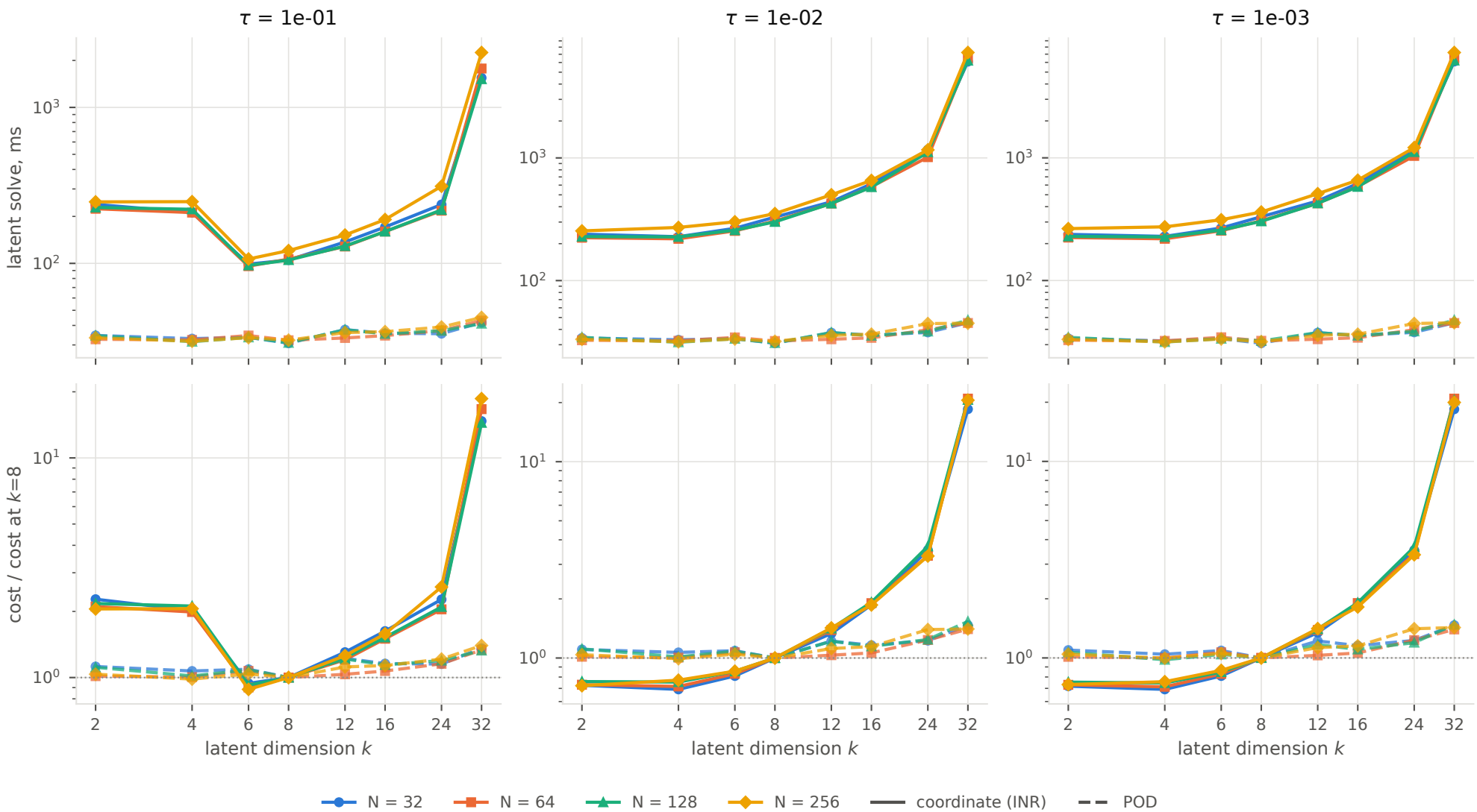
Burgers 2D: cost of the latent solve vs k , overlaid across mesh bottom row normalised at k=8 -- curves collapsing means the k dependence is mesh independent
