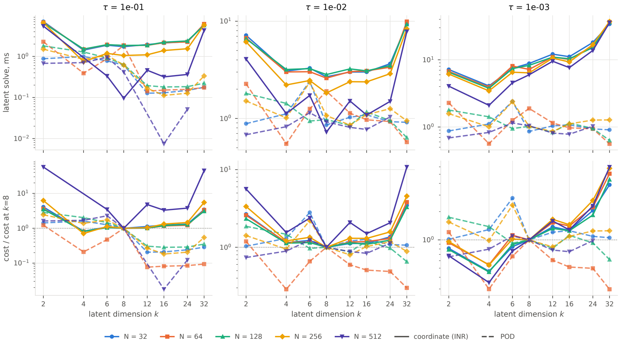
Poisson 2D: cost of the latent solve vs k , overlaid across mesh bottom row normalised at k=8 -- curves collapsing means the k dependence is mesh independent
