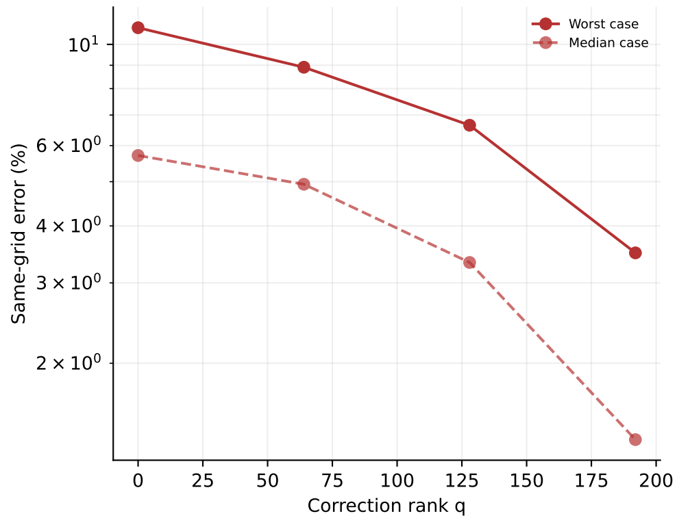
Burgers 3D — 33 nodes per axis — development
