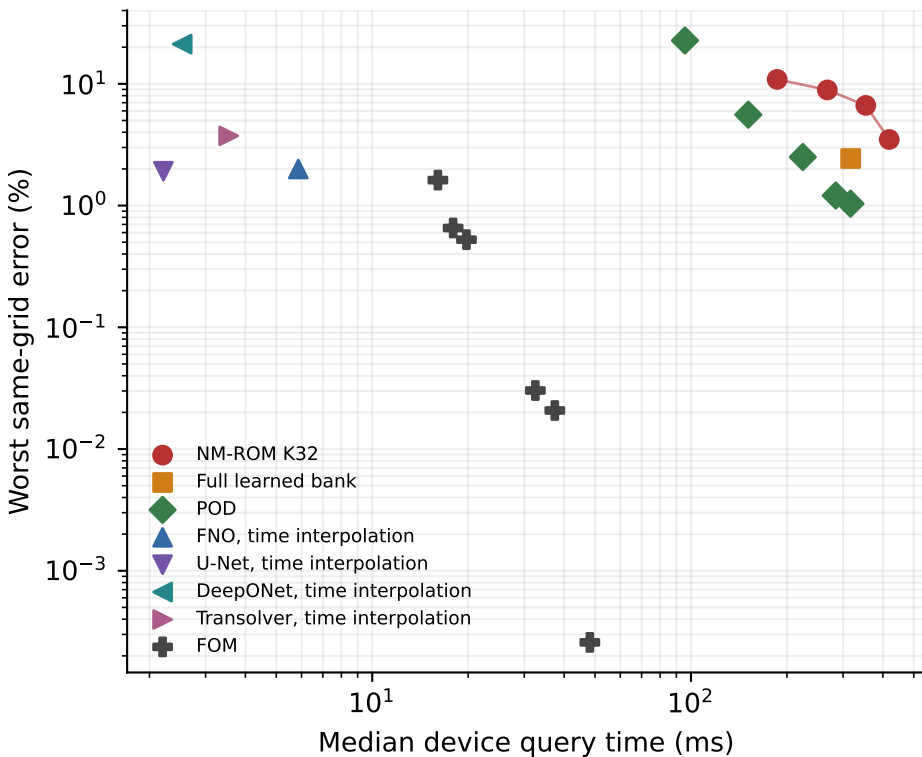
Burgers 3D — 33 nodes per axis — development
