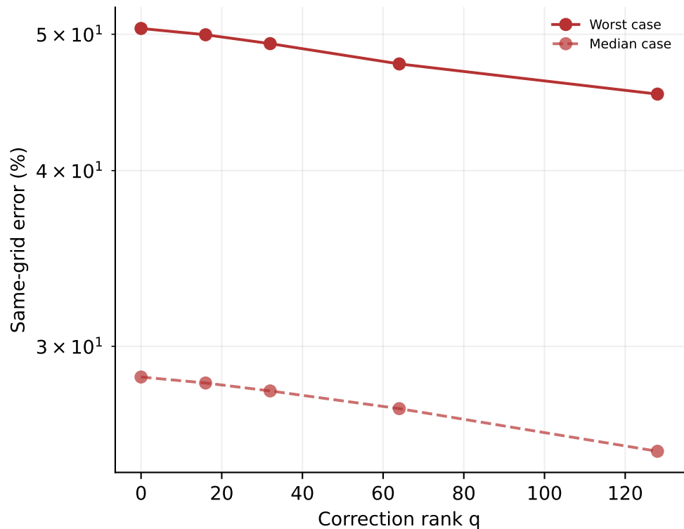
Navier-Stokes 3D — 32 periodic points per axis — development
