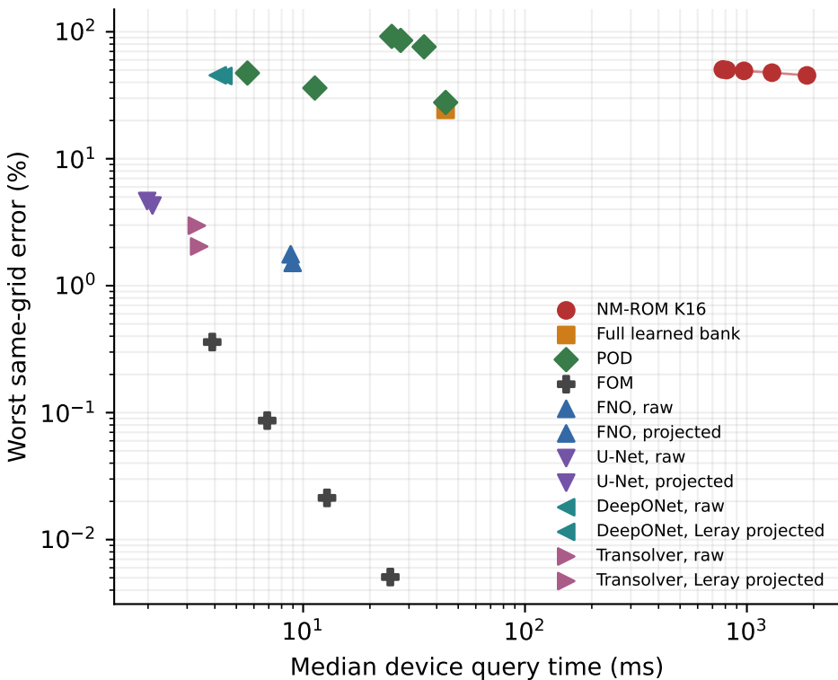
Navier-Stokes 3D — 32 periodic points per axis — development
