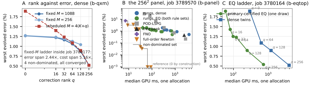
Figure M.1: Burgers2D correction and quadrature studies. A: fixed and scheduled test counts. B: the paired accuracy–cost comparison. C: quadrature and dense residual evaluation. All axes use the recorded experiment’s error and timing definitions.
