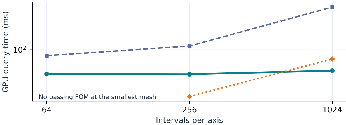
Burgers 2D
