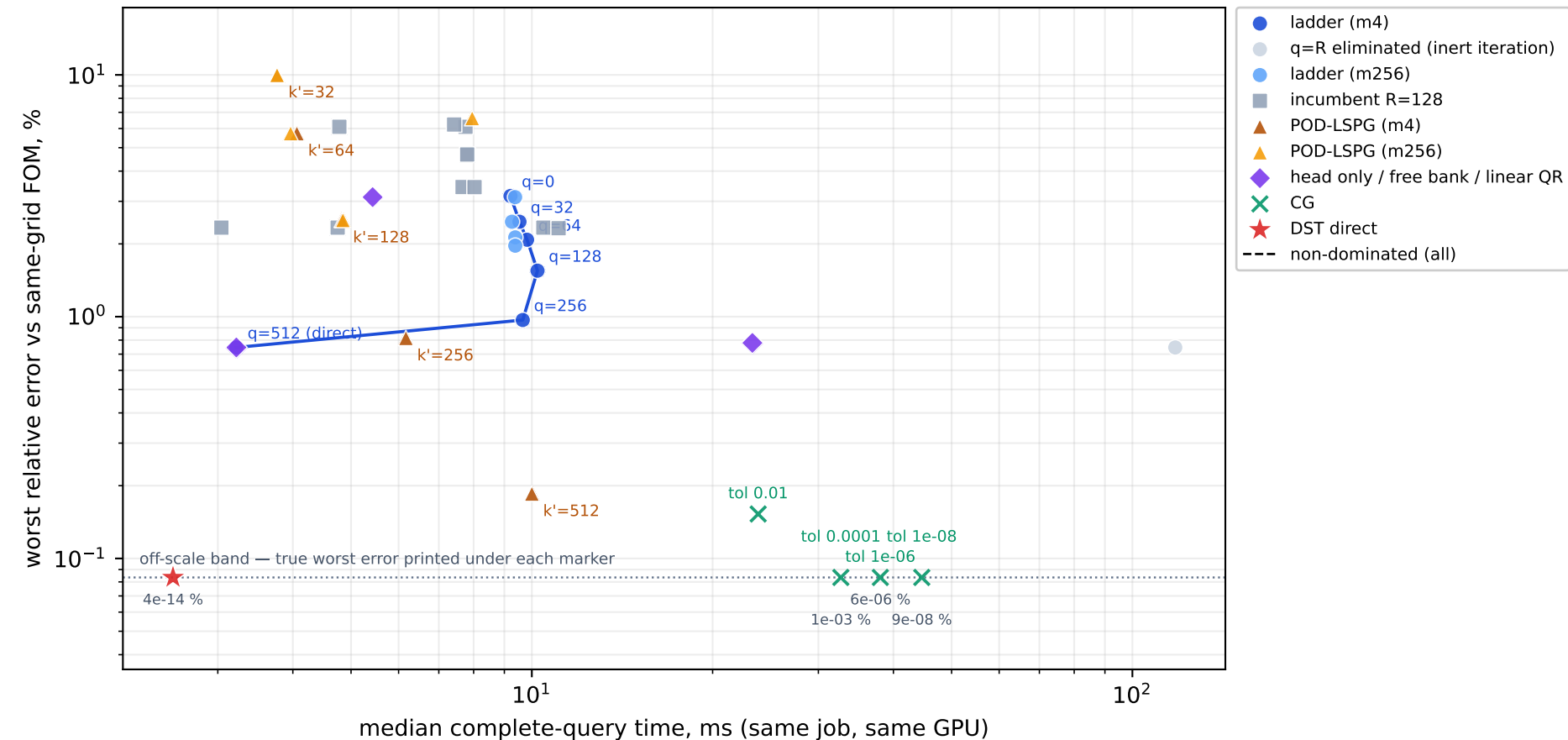
Poisson 2D, 256 2 intervals: correction ladder against every comparator (one job, one GPU, 12 development sources, 3 timed repetitions)
