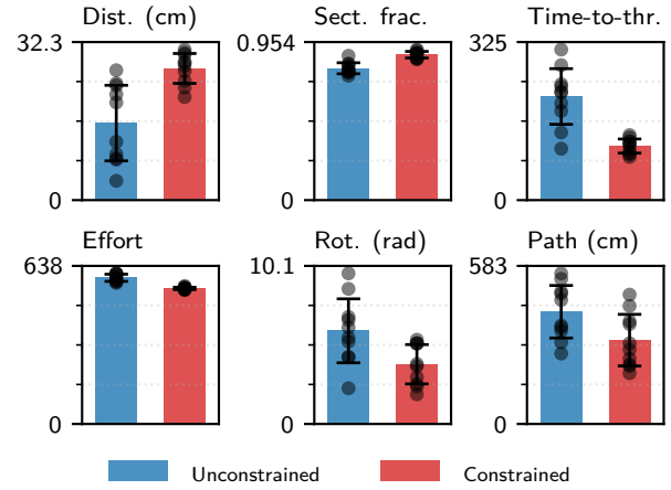
Figure 15: Unconstrained versus anatomically constrained elbow ( \theta_{el} \in [0, \pi] ); setup and encoding as Figure 14. Unconstrained final distance 15.8 \pm 7.7 cm (elbow error 29.0^\circ ); constrained 26.9 \pm 3.1 cm (elbow error 5.3^\circ ). Source
