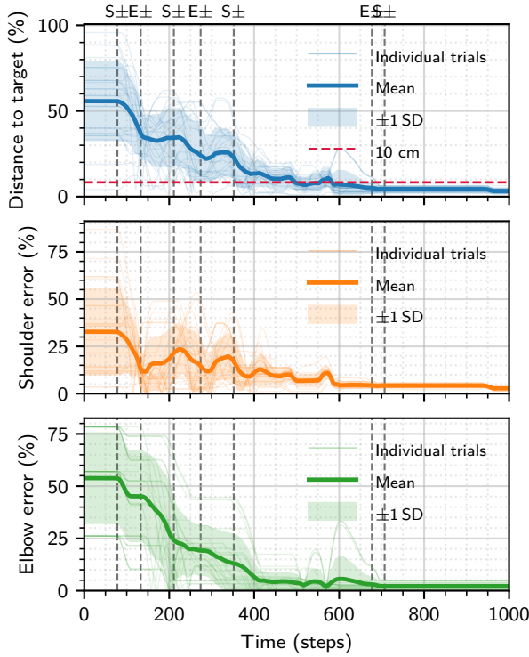
Figure 11: Error time series for the sequential open-loop controller on the 24-target grid (seed 0, T = 1000 steps). Top: distance to target as a percentage of the 120 cm maximum reach. Centre and bottom: shoulder and elbow joint error as a percentage of the 180^\circ maximum wrapped error. Vertical dashed lines mark phase switches in demo trial 7, labelled by the activated phase (S \pm shoulder, E \pm elbow). 24/24 trials reached the 10 cm threshold (mean 309 steps); mean final distance 4.0 cm. Source
