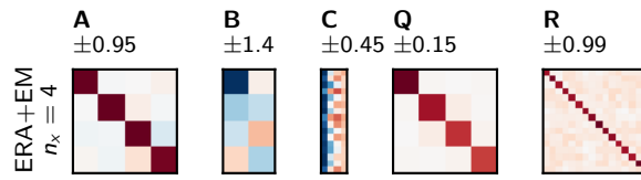
Figure 3: Identified system matrices A , B , C , Q , R of the chosen model. Diverging colour scale is symmetric about zero. Source
