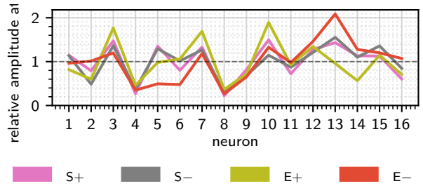
Figure 8: Per-neuron amplitude at each of the four selection frequencies of Figure 7, from sustained open-loop trials ( u_1 = 0.5 + 0.4 \sin(2\pi f^* t) , u_2 = 0.5 ; 1024 steps after 500 burn-in), each profile normalised by its own neuron-mean (dashed line, = 1). Source
