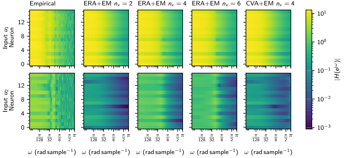
Figure 4: Per-neuron frequency selectivity |H(e^{j\omega})| for inputs u_1 (top row) and u_2 (bottom row), all neurons against \omega \in [0, \pi] on a shared logarithmic colour scale. Leftmost column: empirical response (single-run OLS, 5000 steps, DFT zero-padded to 512 points). Remaining columns: analytic ERA+EM responses for n_x \in \{2, 4, 6\} and CVA+EM at n_x = 4 for comparison. Source
