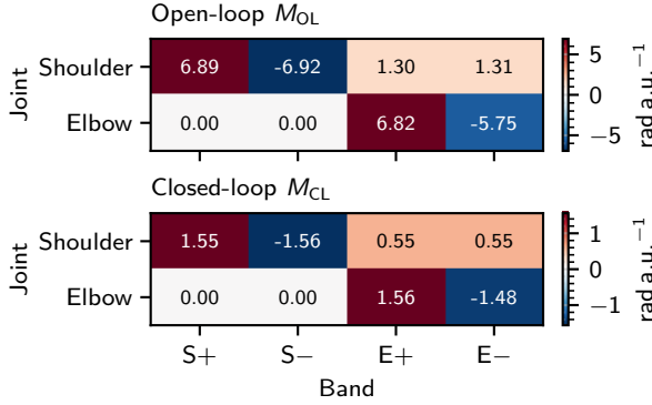
Figure 9: Gain matrices M_{OL}, M_{CL} \in \mathbb{R}^{2 \times 4} calibrated from open-loop (OL) and closed-loop LQI (CL) trials ( T = 800 steps, warmup 200 steps, seed 0). Source
