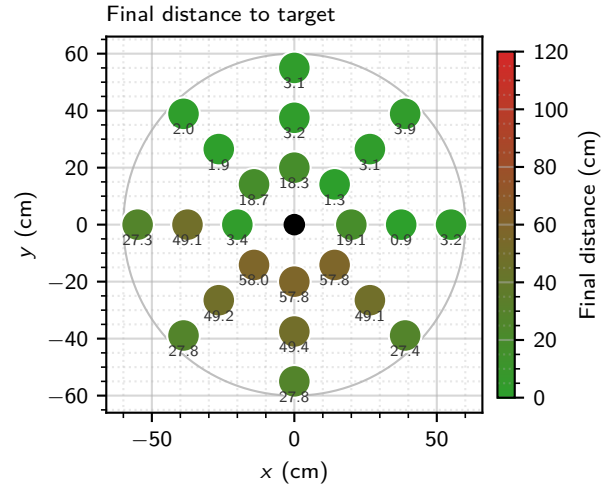
Figure 16: As Figure 12 , but for the controller re-optimised with the elbow anatomically constrained ( \theta_{el} \in [0, \pi] ) via an independent TPE search (150 trials). Source
