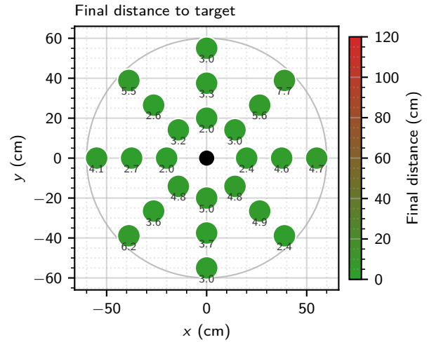
Figure 12: Final distance to target at each location of the 24-target grid (seed 0). The faint circle marks the arm reach boundary ( 2L , twice the link length). Source
