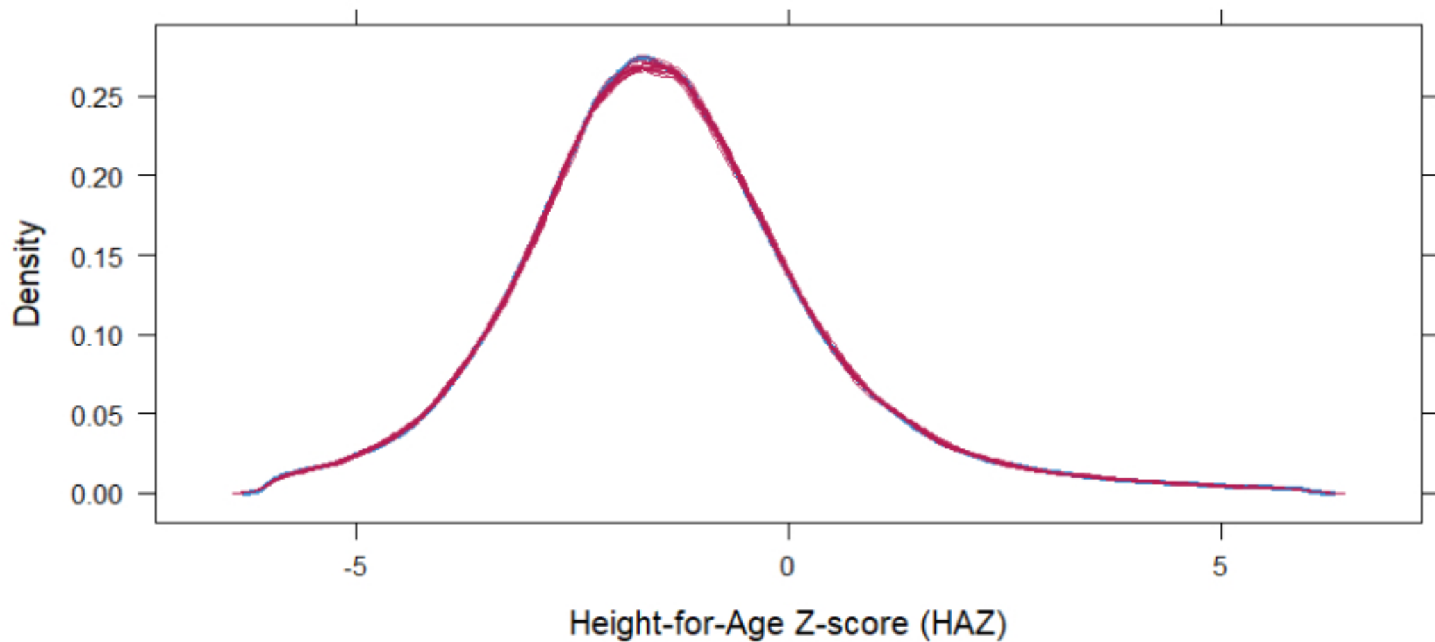
Observed vs Imputed HAZ Distribution (Predictive Mean Matching, m = 20 )
