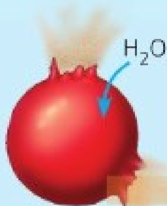
Hypotonic solution
