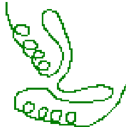
Secondary structure
