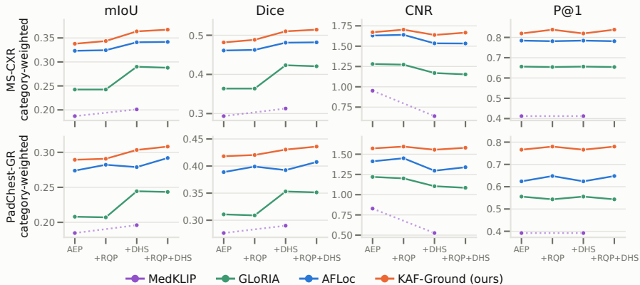
All four metrics across the evaluation protocol, both benchmarks
