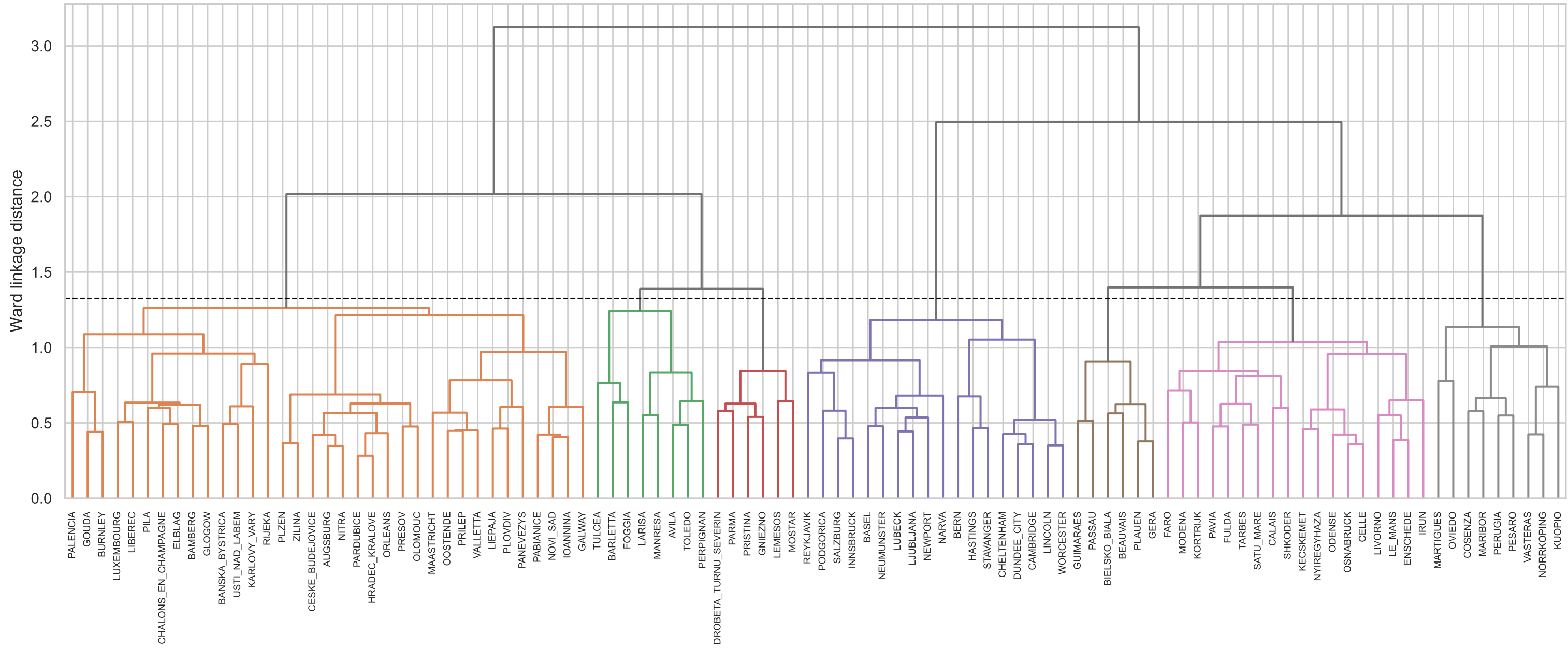
Original-space Ward clustering of exact support profiles (k=7)
