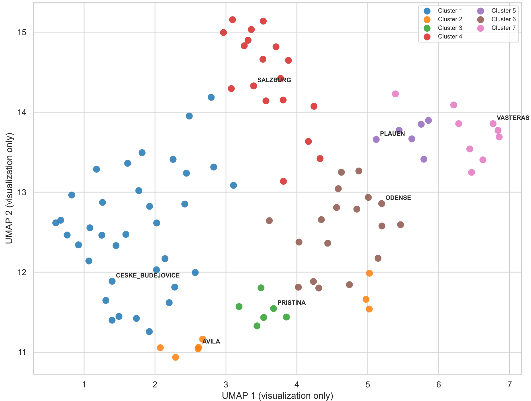
UMAP visualization colored by fixed original-space clusters n_neighbors=15, min_dist=0.1, metric=euclidean, seed=42
