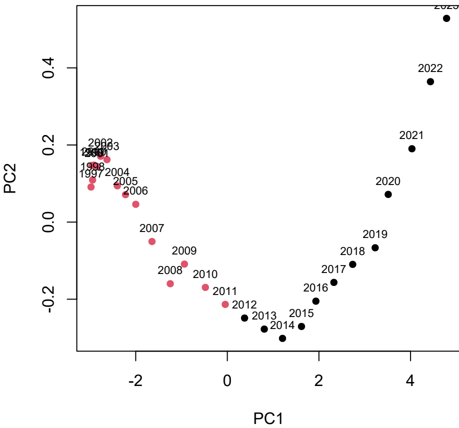
Original data
