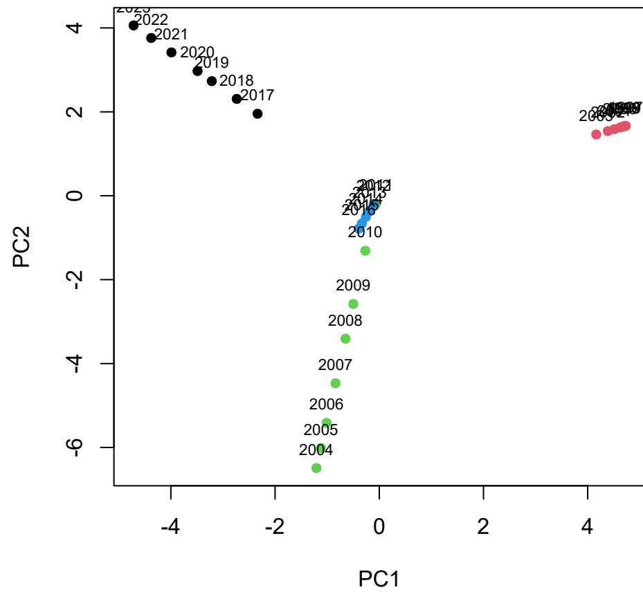
Sparsified data
