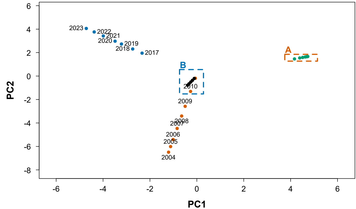
Sparsified representation
