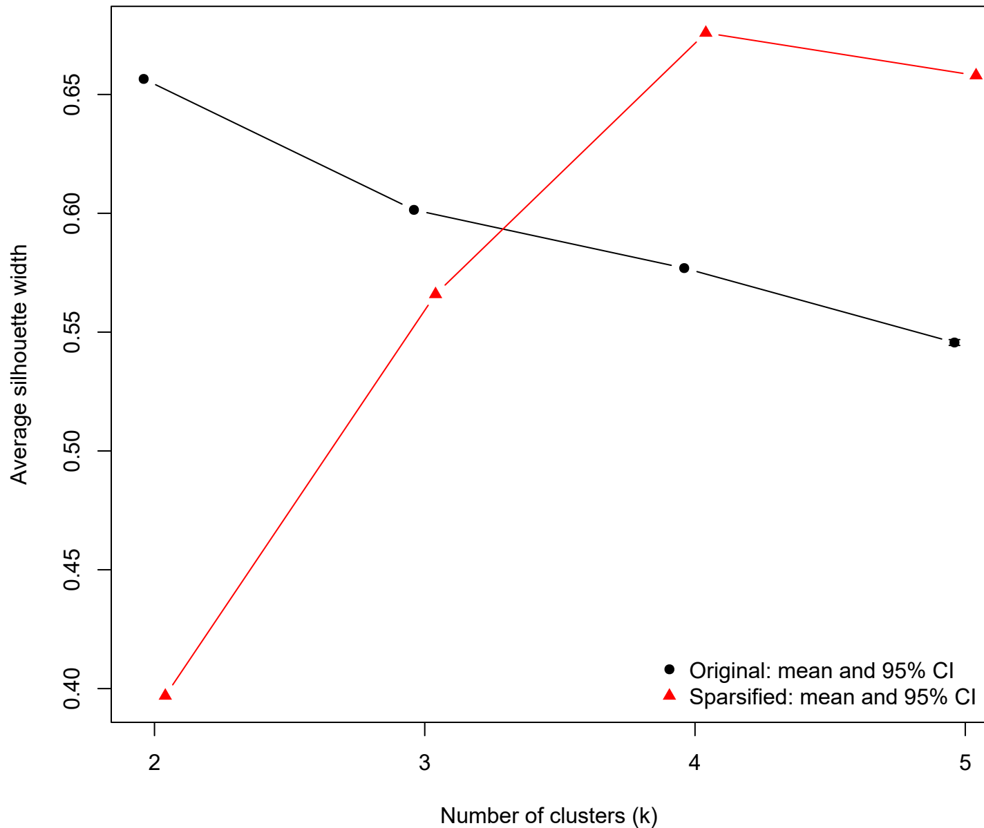
Chinese housing data: repeated k-means
