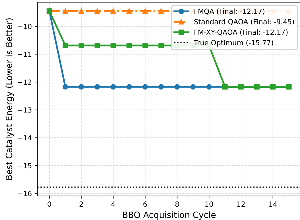
(a) Materials Property Optimization Trajectory
