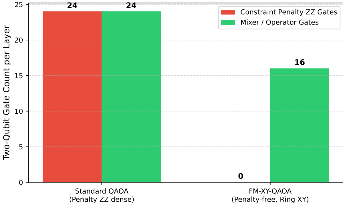
NISQ Hardware Compilation Overhead (N=16)
