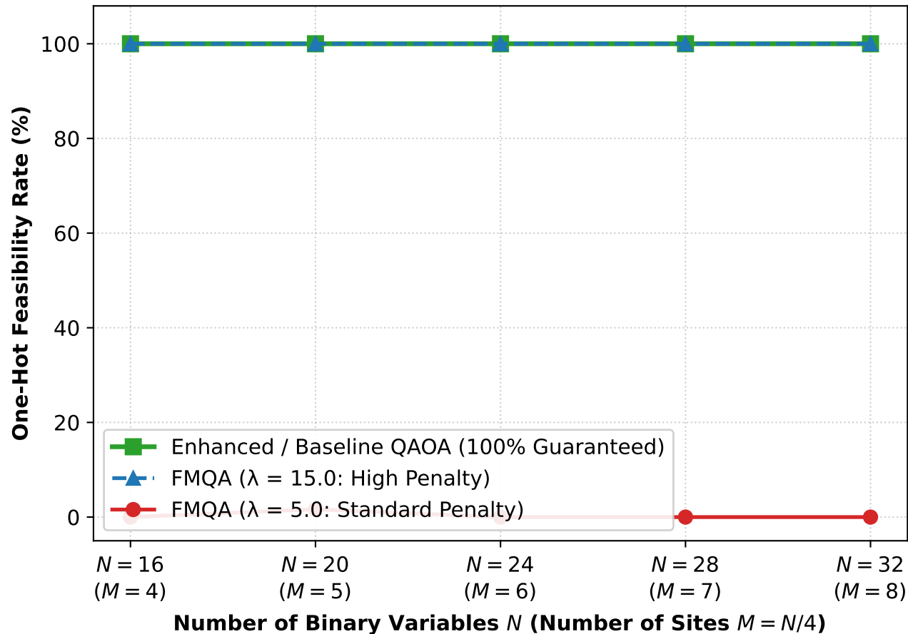
(a) Constraint Feasibility in Multi-Scale Catalyst Model
