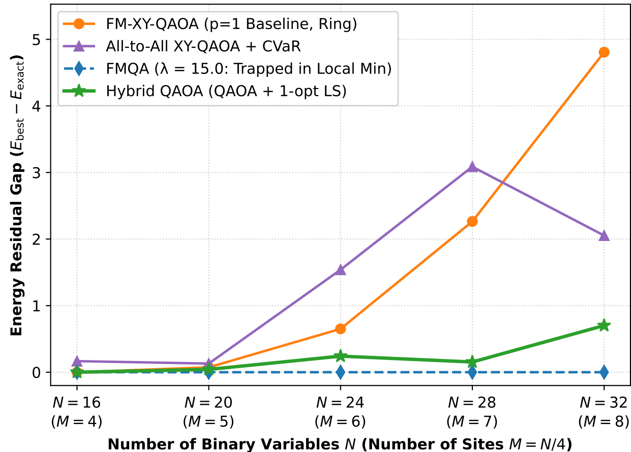
(b) Optimization Residual Gap from True Ground State
