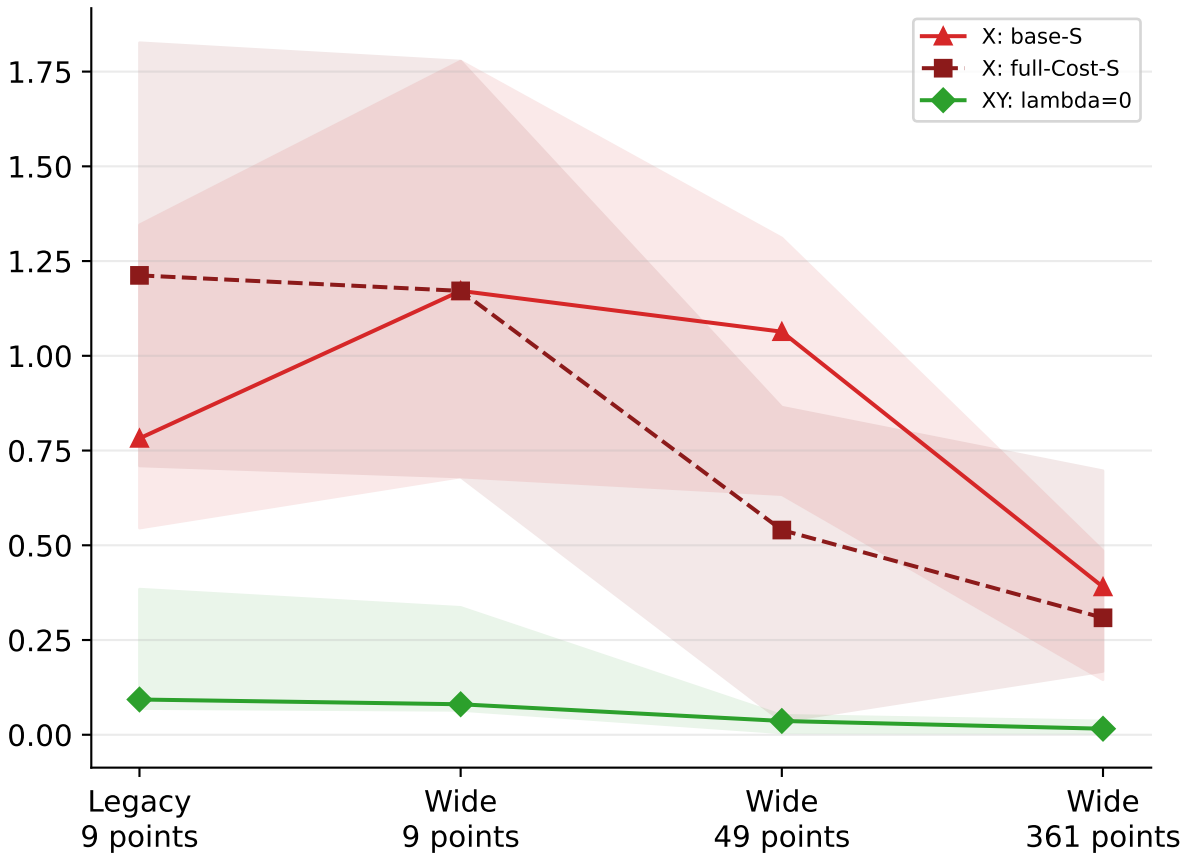
N=6: Conditional best10 FM gap (eV)
