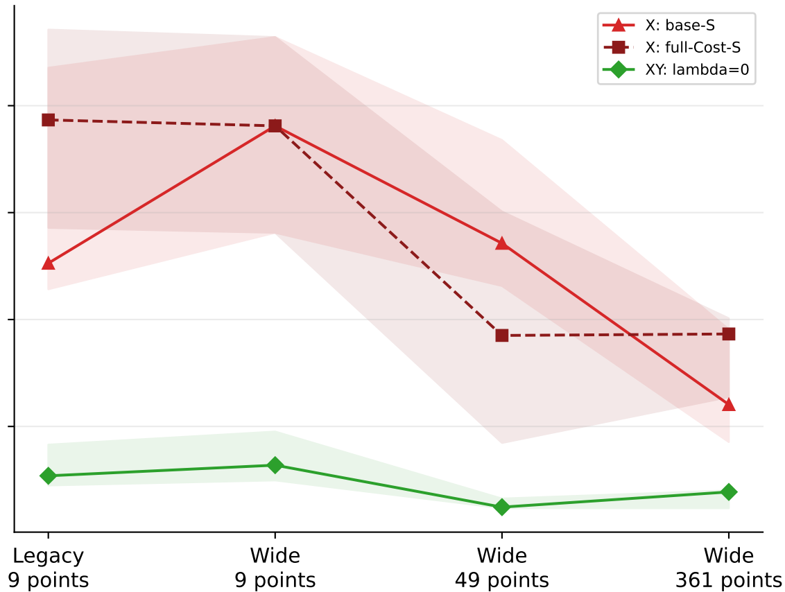
N=9: Conditional best10 FM gap (eV)
