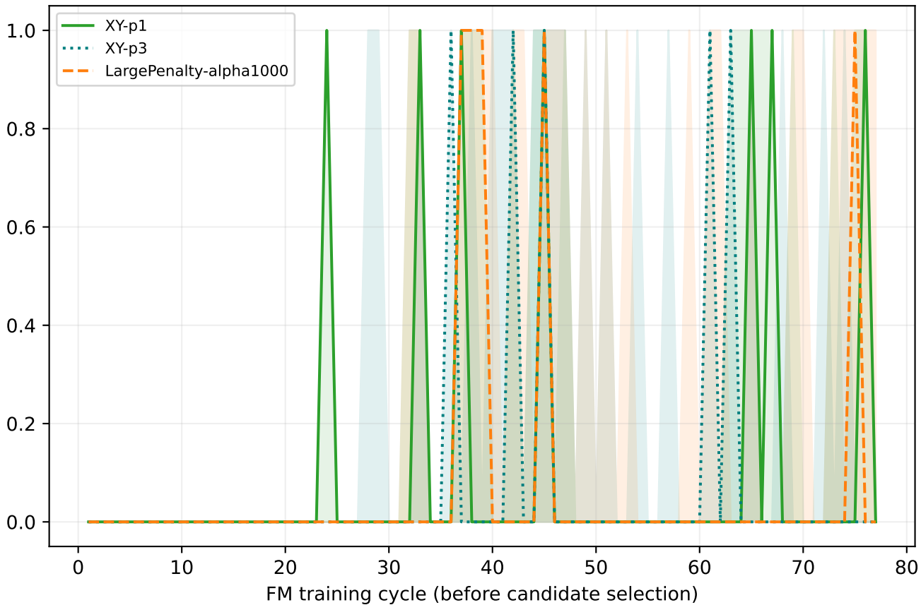
FM argmin contains true optimum
