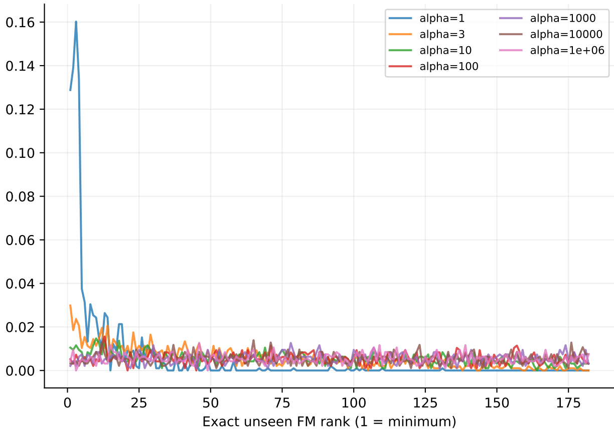
Empirical unseen sample frequency
