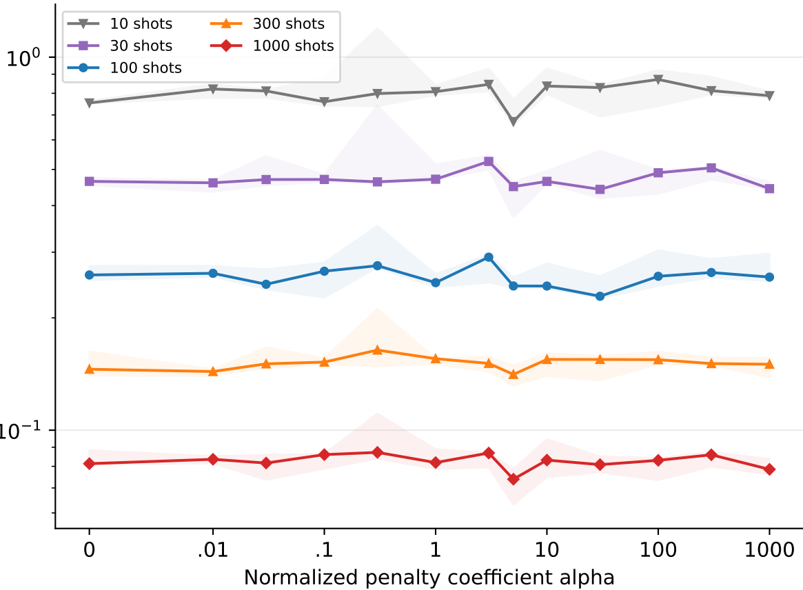
Normalized base-FM energy RMSE
