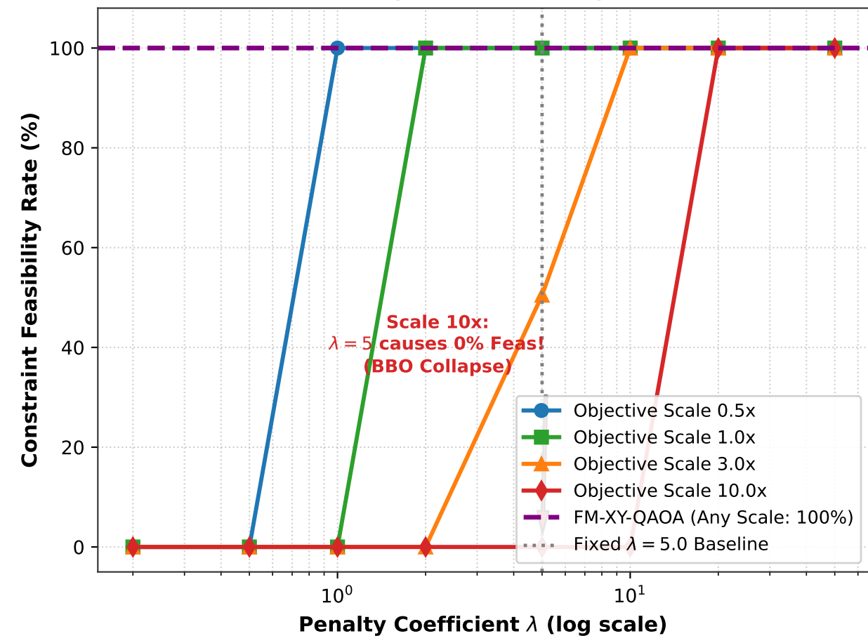
(a) Constraint Feasibility vs \lambda across Objective Scales ( N = 12 )
