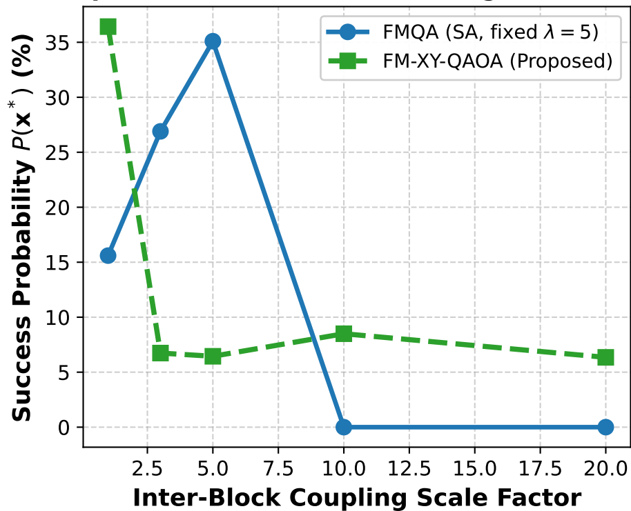
(b) Optimal Success under Heterogeneous Scales
