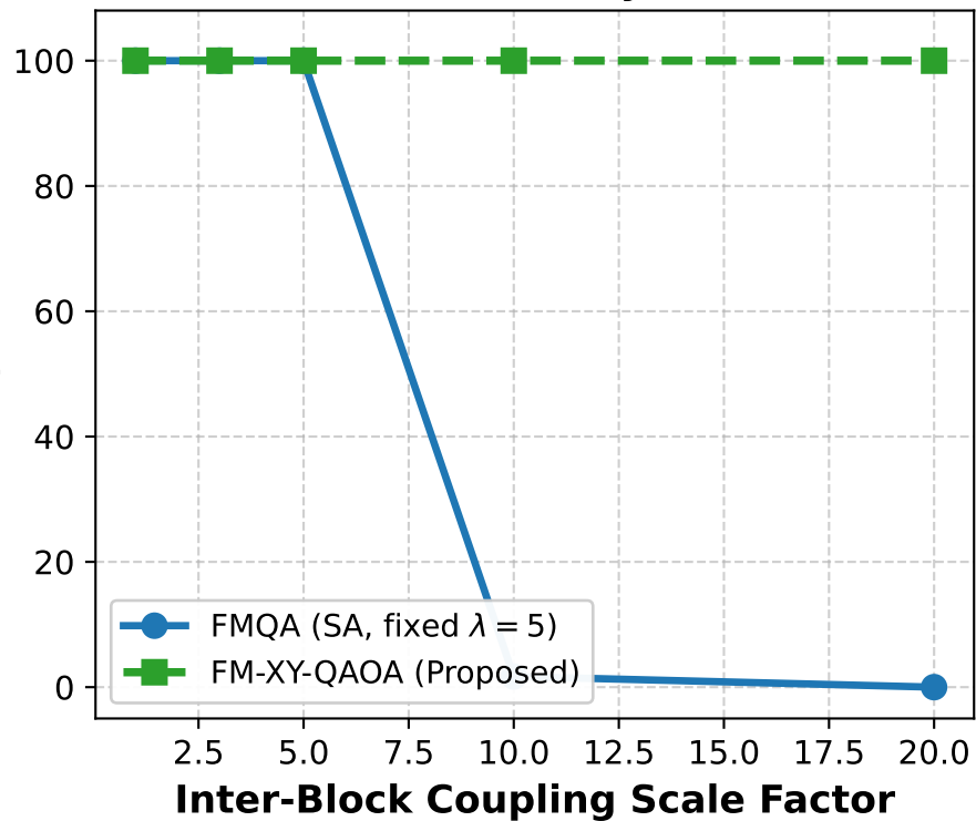
(a) Constraint Feasibility vs Scale Ratio
