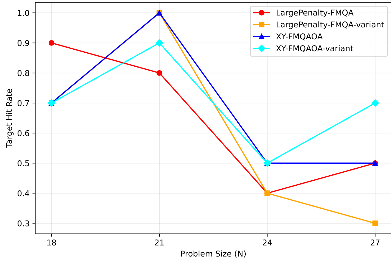
BBO Final Target Rate vs N (BB2)
