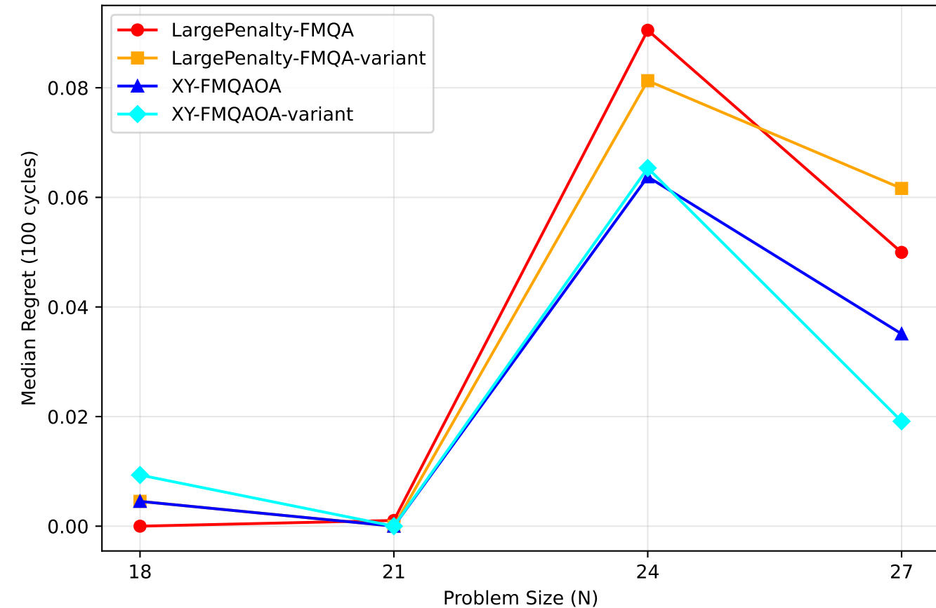
BBO Final Median Regret vs N (BB2)
