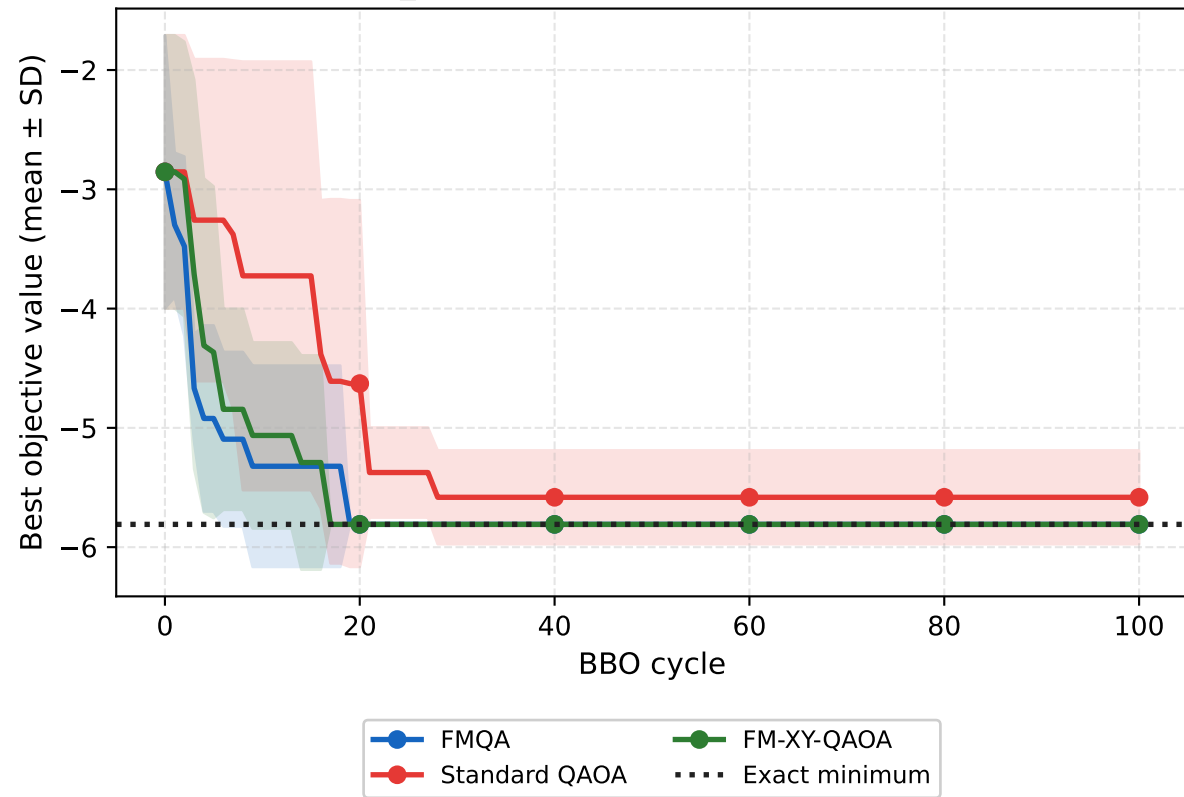
BB2_random: BBO Seed Robustness
