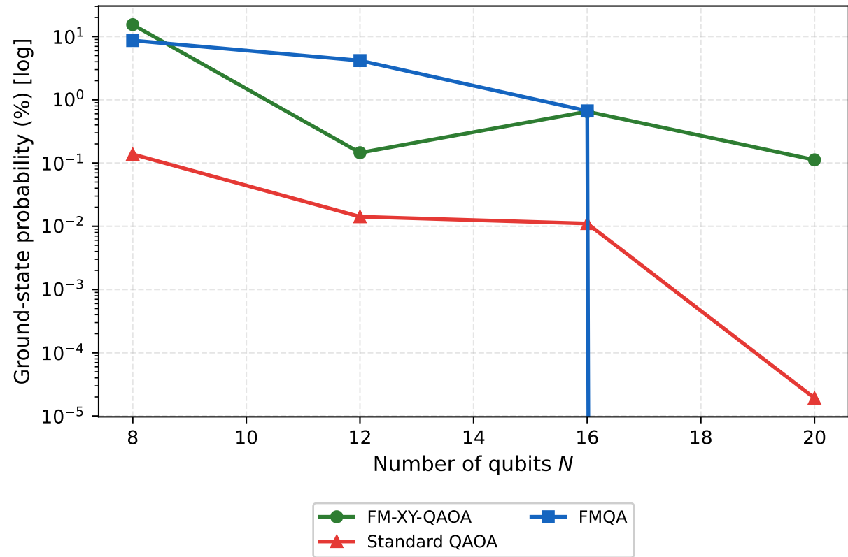
Ground State Probability vs Number of Qubits
