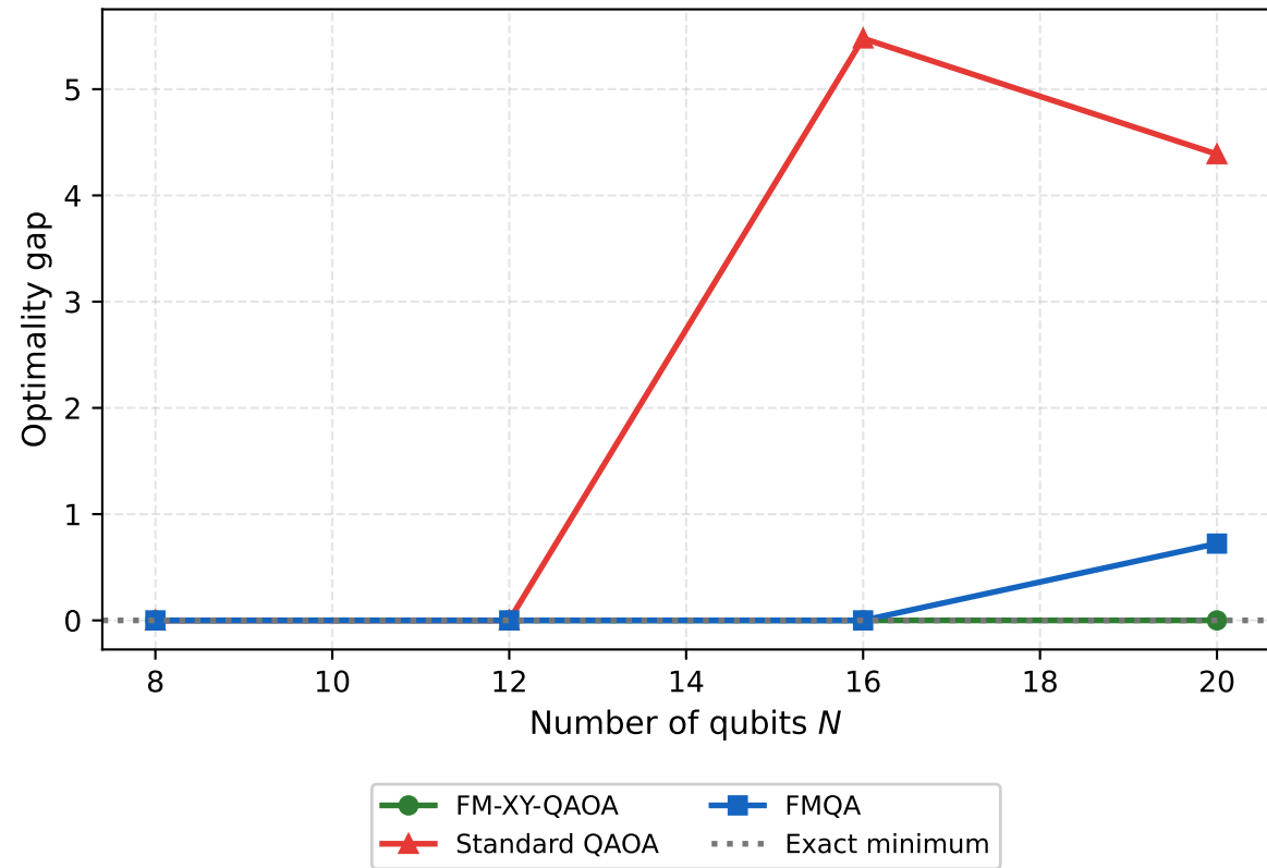
Optimality Gap vs Number of Qubits
