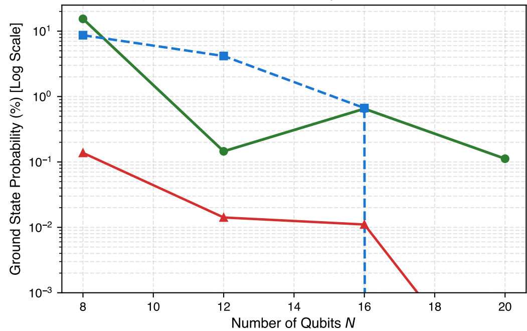
(c) Ground State Hit Probability P(x^*) vs Scale N
