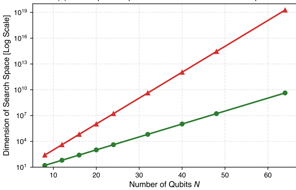
(b) State Space Explosion: Full Hilbert vs Valid Subspace
