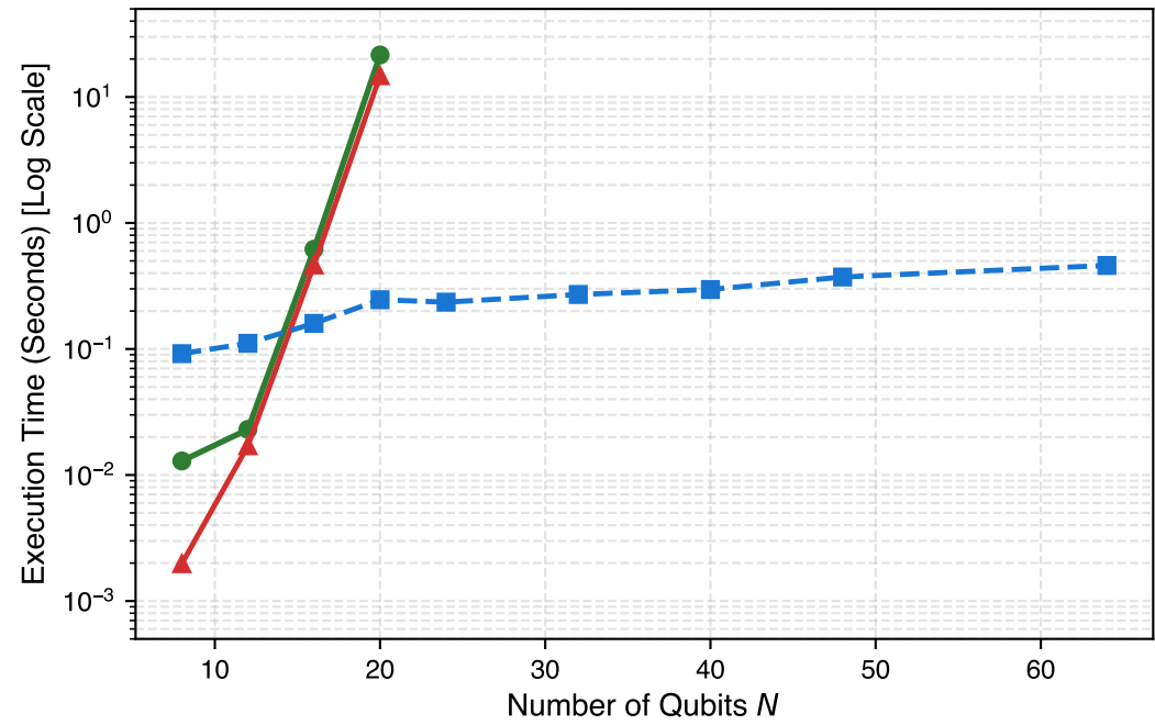
(e) Simulation Runtime Scaling vs Scale N
