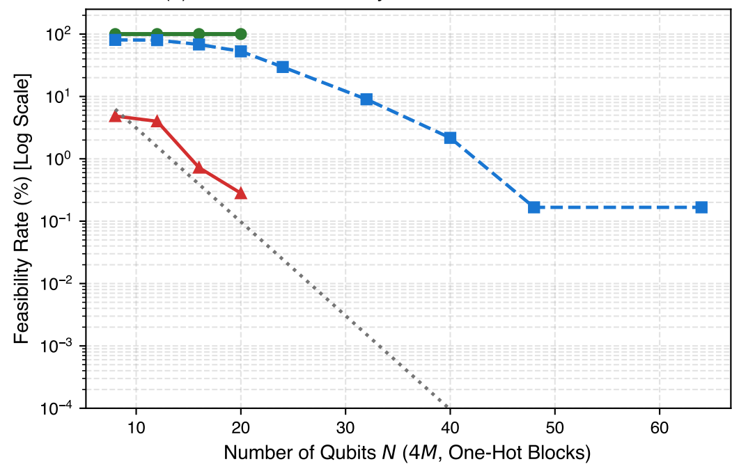
(a) Constraint Feasibility Rate vs Number of Qubits N
