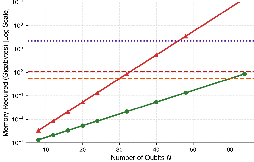
(f) Theoretical RAM Footprint & Classical Limits
