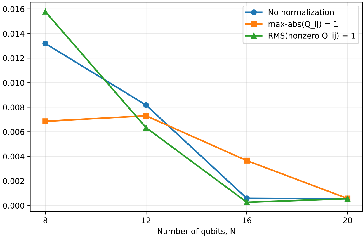
Ground-state probability, P(\text{opt})
