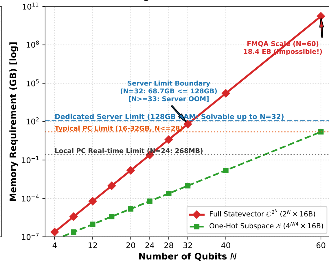
(c) RAM Scaling & Classical Simulation Limits
