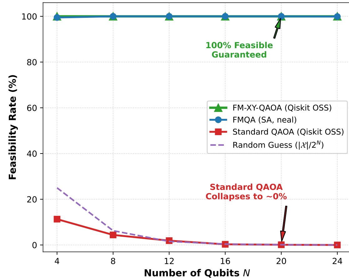
(a) Constraint Satisfaction vs Qubit Scale
