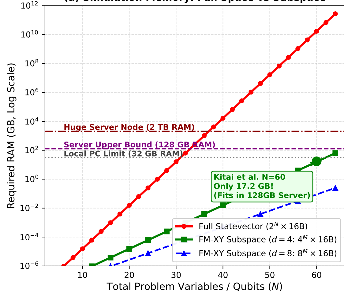
(a) Simulation Memory: Full Space vs Subspace
