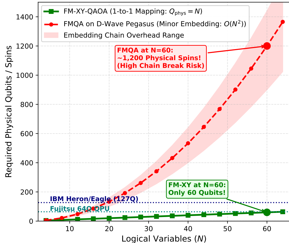
(c) Physical Hardware Qubit Overhead
