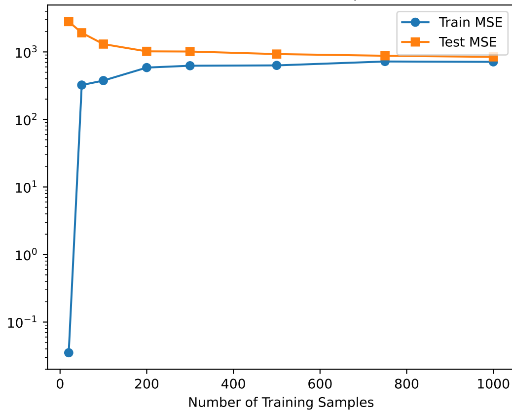
Variant FM (Huber+L2, Ep 200)
