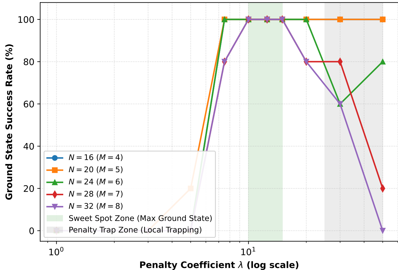
(b) Ground State Success Rate vs Penalty \lambda
