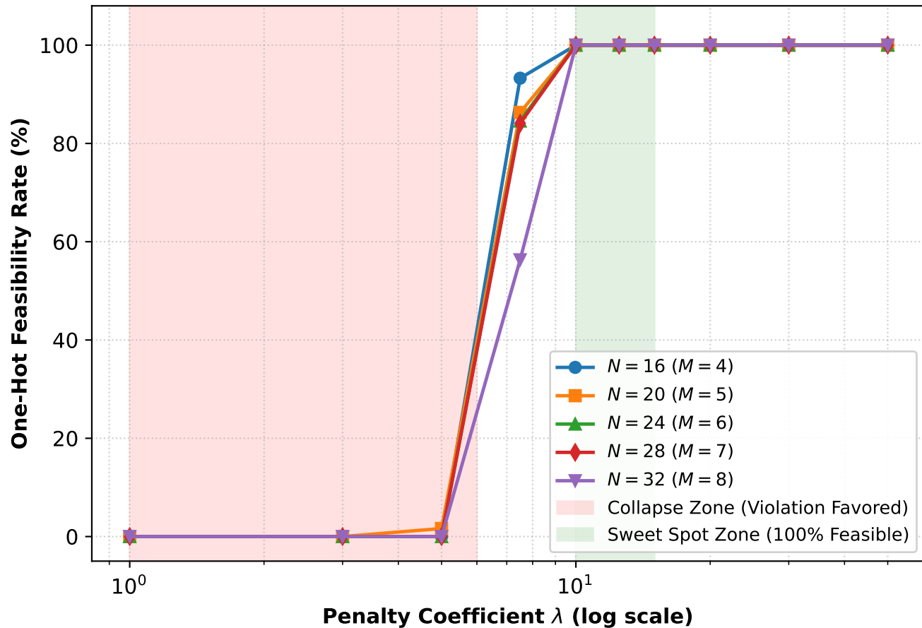
(a) Constraint Feasibility vs Penalty \lambda
