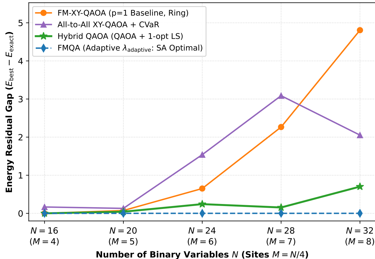
(b) Optimization Residual Gap from Ground State
